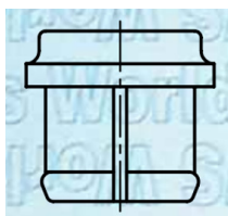
TIP SEAL, II BLACK SILICONE 180° NWW # II-SI QUANTITY 2800
