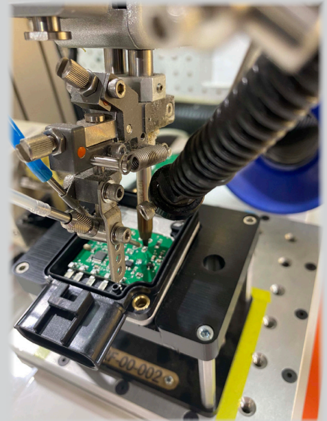
ROBOTIC SOLDERING
