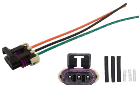
Walker # 270-1036 3-Wire
