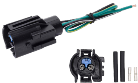
Walker # 270-1049 2-Wire
