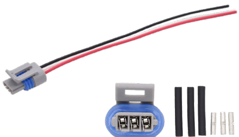
Walker # 270-1039 3-Wire
