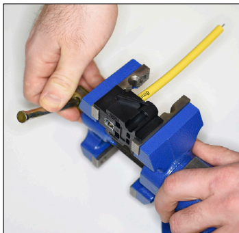
Crimping
