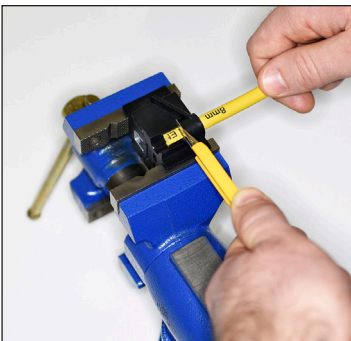
Stripping
