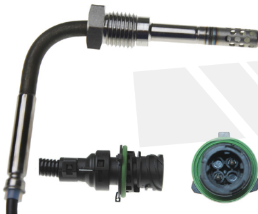
1003-1004 Harness Length = 12.5" / 315mm
