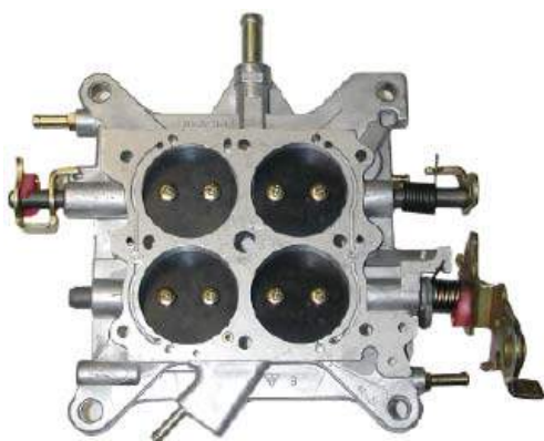
85-673 BASE PLATE COMPLETE ASSEMBLY (Model: 4779)
