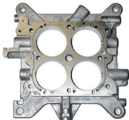
85-580 BARE BASE PLATE ASSEMBLY (Model: 4777, 4778, 4779, 4780)
