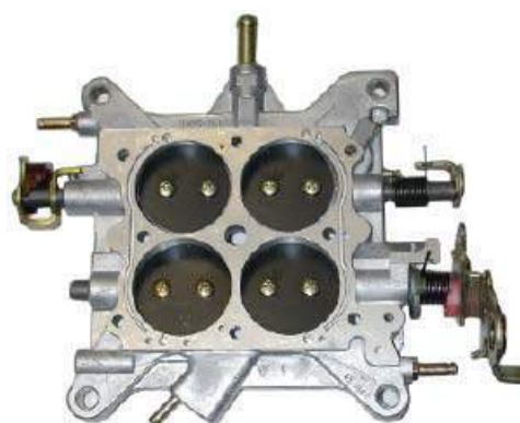
85-674 BASE PLATE COMPLETE ASSEMBLY (Model: 4781)
