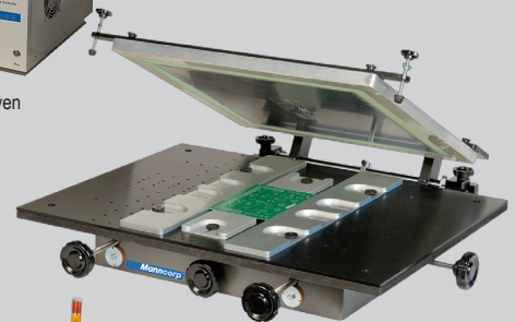
Stencil Printer
