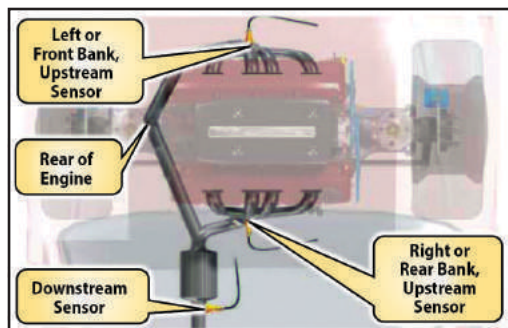
V6 & V8 - TRANSVERSE *
