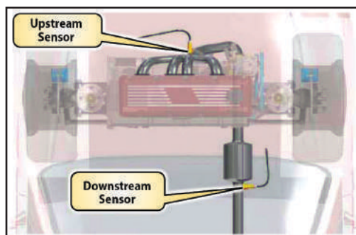
L4 & L6 - TRANSVERSE *
