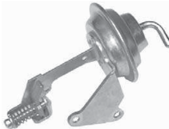
101-932 (R-2, R-4) BUICK (8) 1977-90 CADILLAC (6, 8) 1981-90 CHEVROLET (8) 1986-90 CHEV/GMC TRUCK (8) 1977-78 OLDSMOBILE (8) 1975-90 PONTIAC (8) 1977-81, 1986-90
