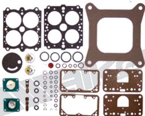
19055 (H-4) HOLLEY UNIVERSAL
