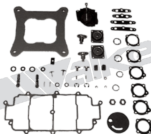
151095 (H-4) HOLLEY PERFORMANCE CARB 4010 SERIES
