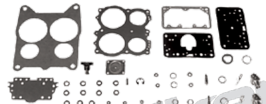
19048 (H-4) OMC # 987313
