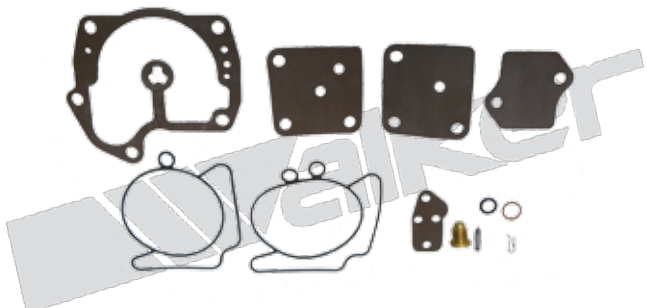
16038V (JOHNSON) JOHNSON-EVINRUDE 120.0 H.P. TO 300.0 H.P. JOHNSON-EVINRUDE # 435676, 435678, 435752, 437327, 438079, 439079
