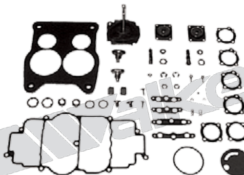
151096 (H-4) HOLLEY PERFORMANCE CARB 4011 SERIES VOLVO PENTA (8)
