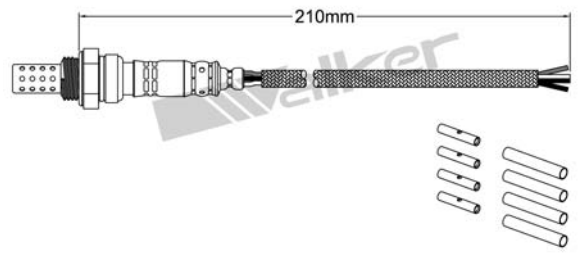
250-24200 UNIVERSAL FOUR WIRE
