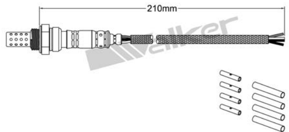
250-24000 UNIVERSAL FOUR WIRE
