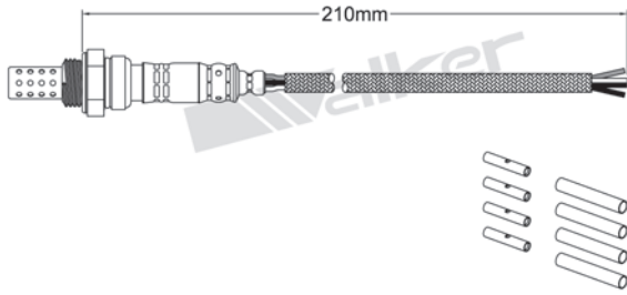
250-24400 UNIVERSAL FOUR WIRE
