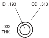
236F NEEDLE VALVE WASHER
