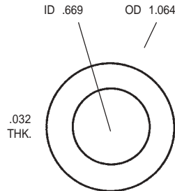
25F BRASS SKID WASHER
