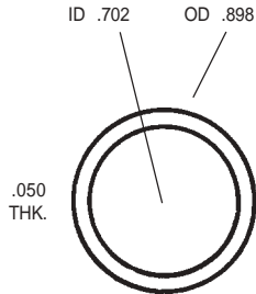
236F NEEDLE VALVE WASHER
