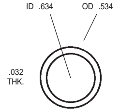
34F COPPER TOP JET WASHER
