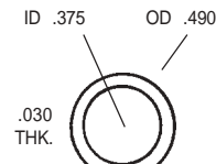
G52 DRAIN PLUG WASHER
