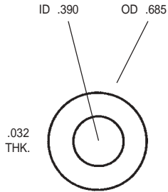
40F JET GLAND WASHER
