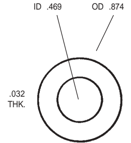
34F COPPER TOP JET WASHER
