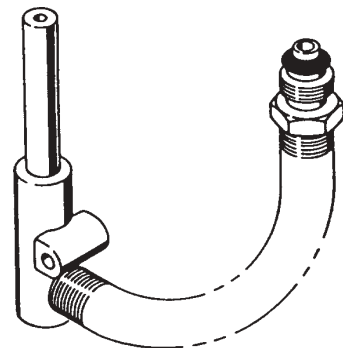
125-2 MAIN JET ASSEMBLY
