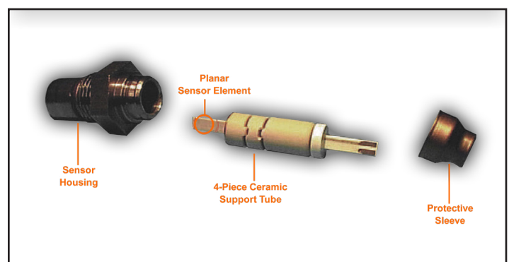
The planar type uses a much lighter unified strip to produce voltage instead of that big thimble. With its integrated heater, it starts sending the ECM accurate signals almost immediately upon start-up (courtesy Robert Bosch).
