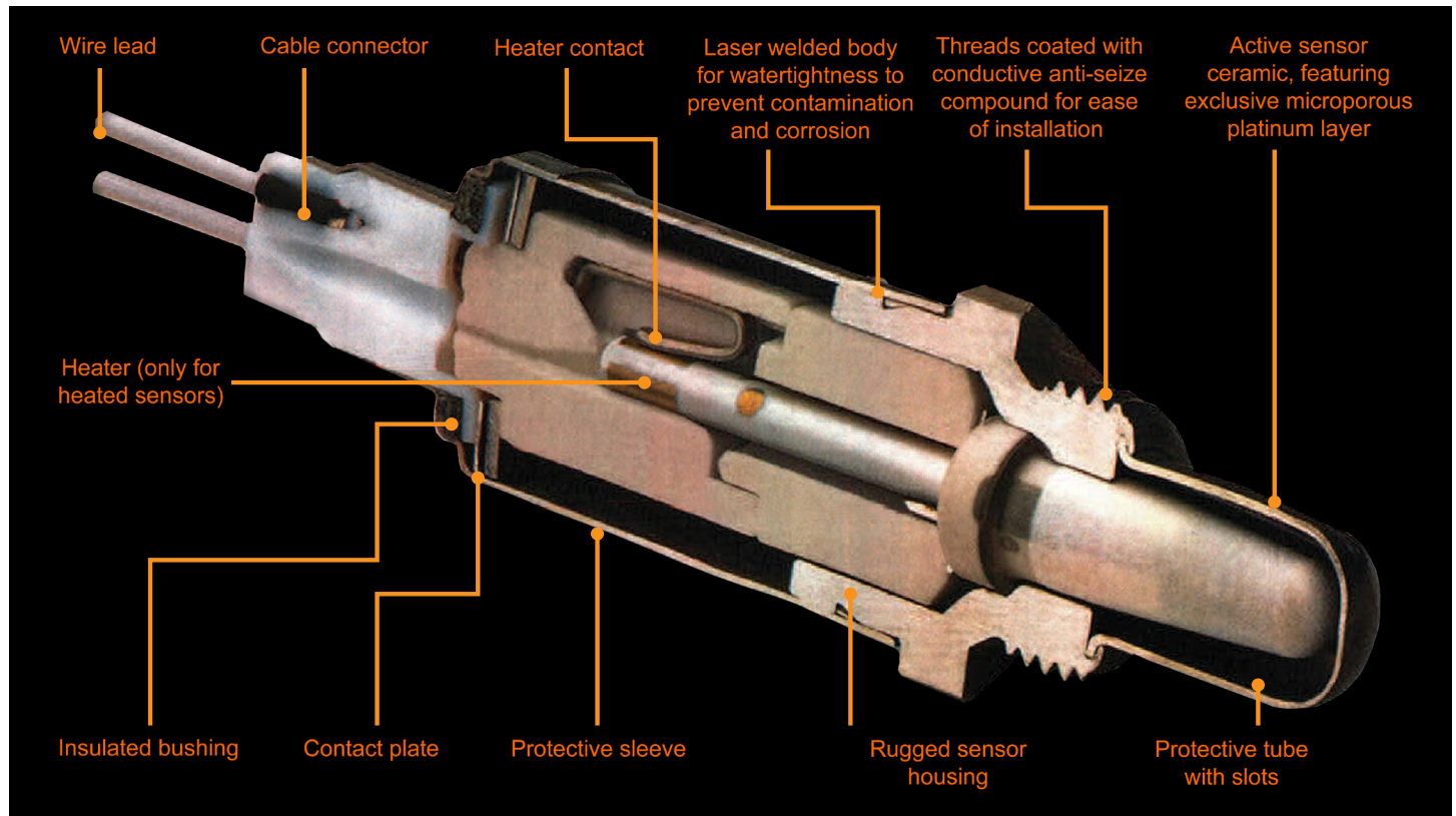
The ceramic thimble with its metallic coating acts as a galvanic cell. The difference in the oxygen content of the reference air to that of exhaust gas is what generates voltage (courtesy Robert Bosch).
