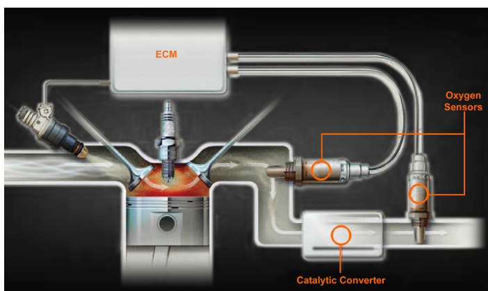
The addition of an oxygen sensor downstream of the catalytic converter makes it possible for second-generation on-board diagnostics to test the catalyst's capacity and efficiency (courtesy Robert Bosch).
